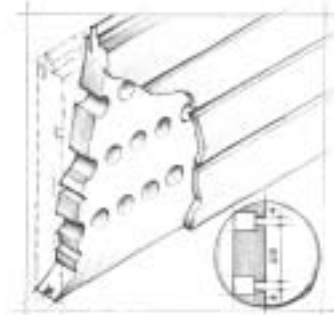
Tipologia 28/4 Perforazione 7.5% Type 28/4 7.5% drilling
